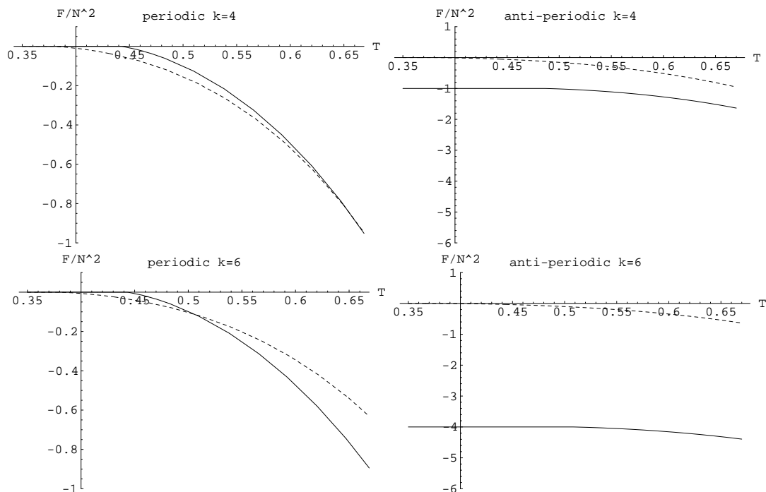
Figure 1: Free energies F(T)/N^2 as functions of T in the cases with the periodic and the anti-periodic boundary conditions and with k = 4, 6 . The solid lines are for the trivial holonomy case and the dotted lines are for the \mathbb{Z}_k symmetric case.
